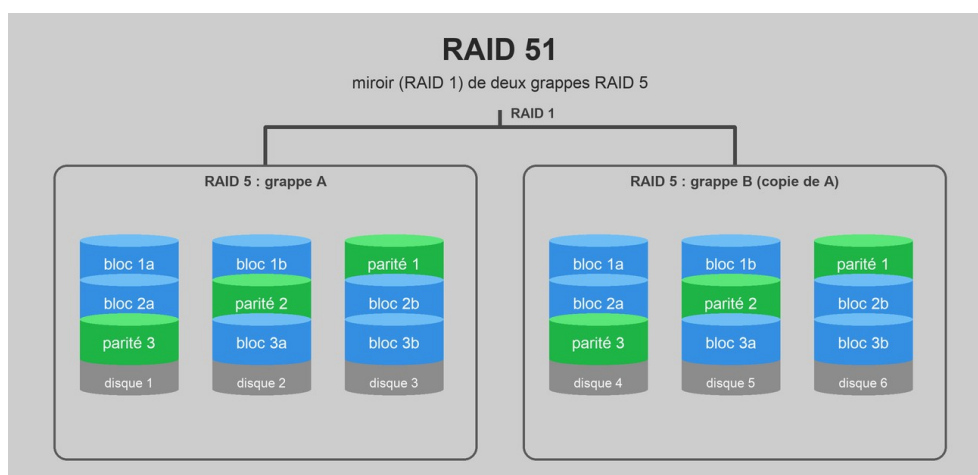
Figure 9 : RAID 51
