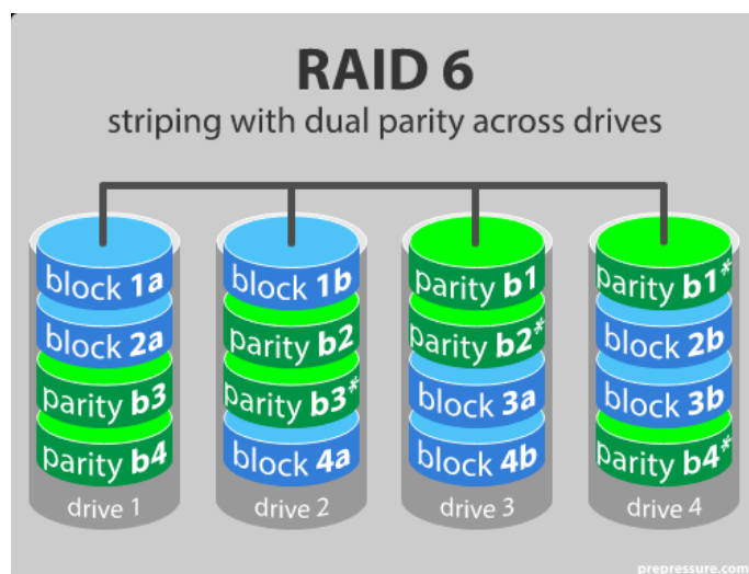
Figure 7 : RAID 6
